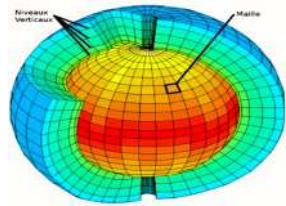
3D-EnVar AROME
