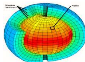
3D-EnVar AROME
